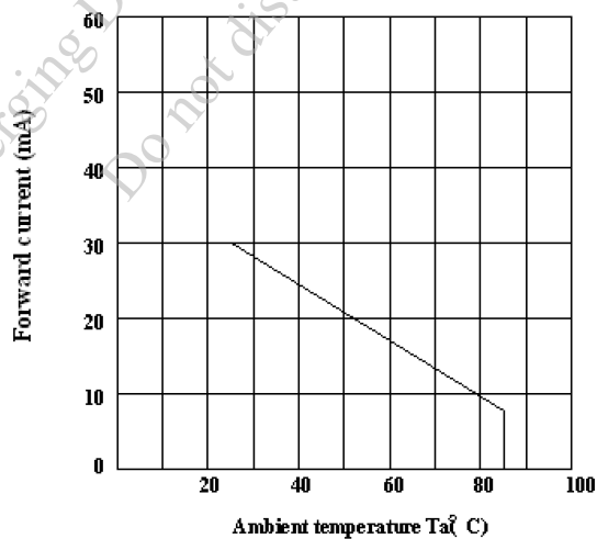
Forward current derating curve vs. ambient temperature
