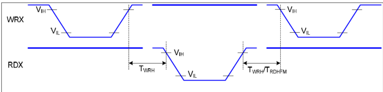
Figure 4 Write-to-read and read-to-write timing
