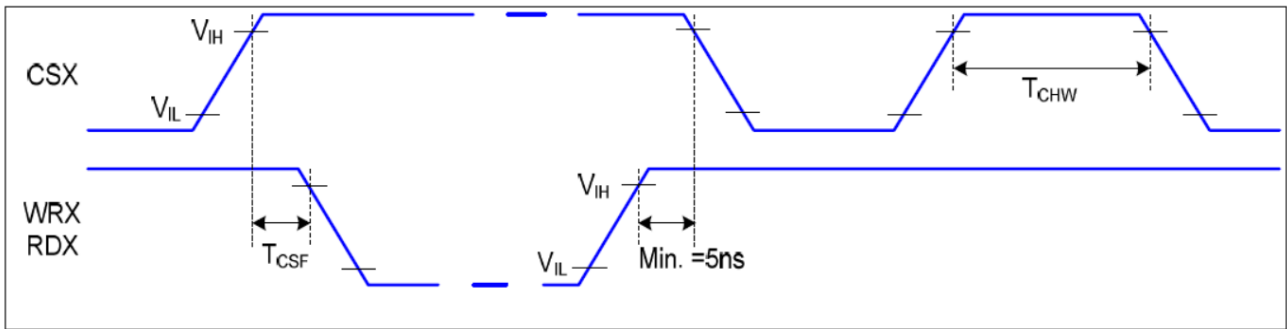
Figure 3 Chip selection (CSX) timing
