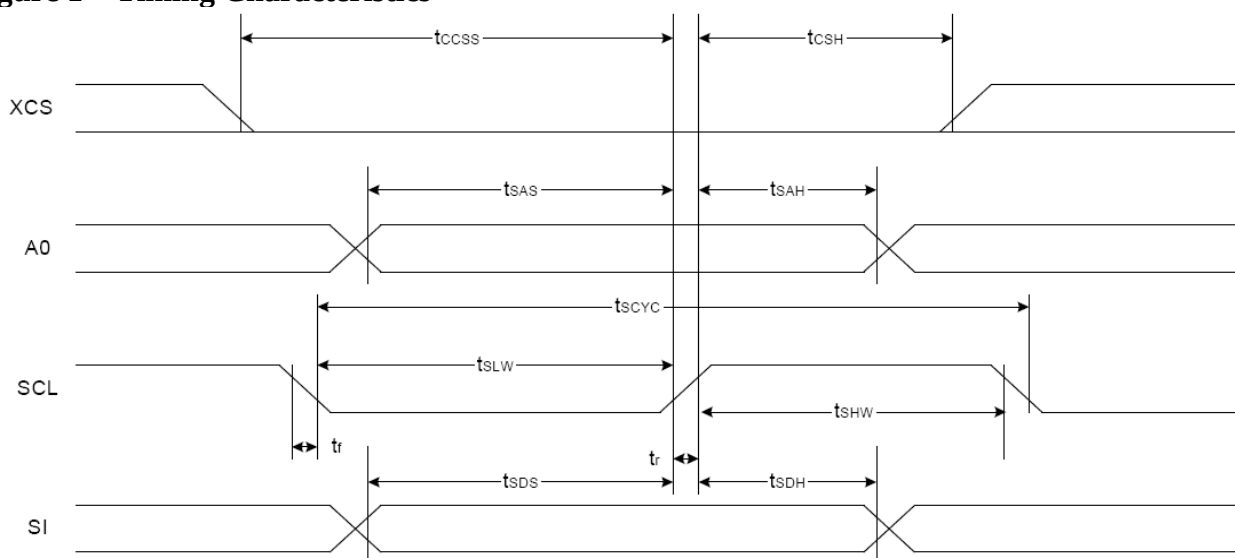
Figure 1 Timing Characteristics
