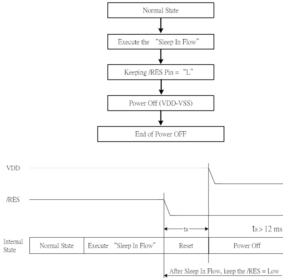
Figure 8.2.8.1 Power off
